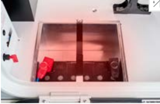
Heated battery centre with main battery switch; Standard: Gel batteries 1 x 80 Ah, extendible to 2 x 80 Ah, optional 90 Ah lithium-ion battery including battery computer and separate touch display
